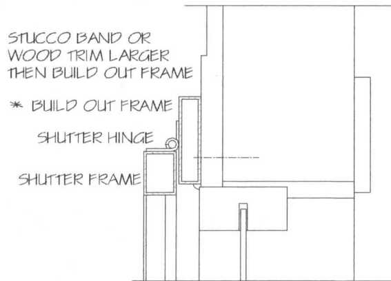
5 STUCCO BAND OR WOOD TRIM BSI LARGER THEN BUILD OUT FRAME
