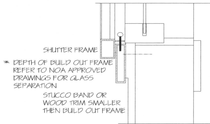
6 STUCCO BAND OR WOOD TRIM BSI SMALLER THEN BUILD OUT FRAME
