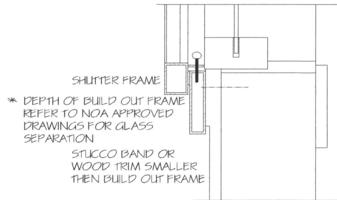
5 STUCCO BAND OR WOOD TRIM BSI SMALLER THEN BUILD OUT FRAME
