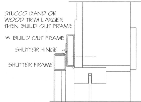
4 STUCCO BAND OR WOOD TRIM BSI LARGER THEN BUILD OUT FRAME
