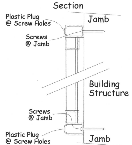
FIGURE 2 - SECTION
