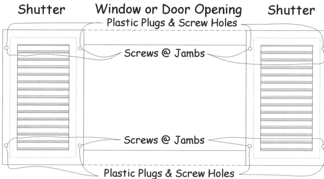
FIGURE 1 - ELEVATION
