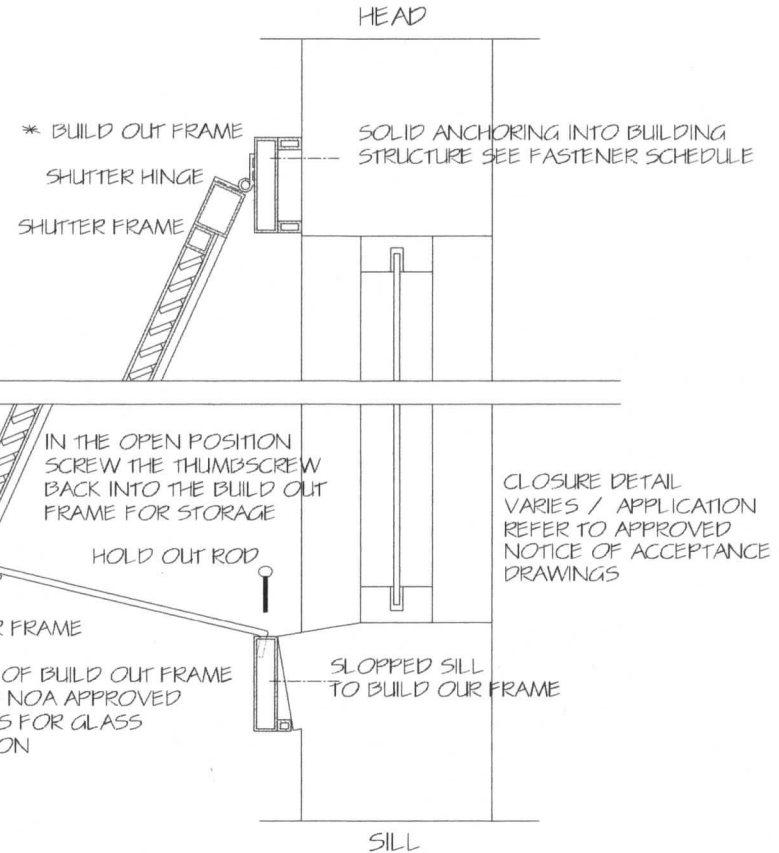
4 HURRICANE BAHAMA OPEN POSITION BSI BUILD OUT FRAME OVER CONC SILL
