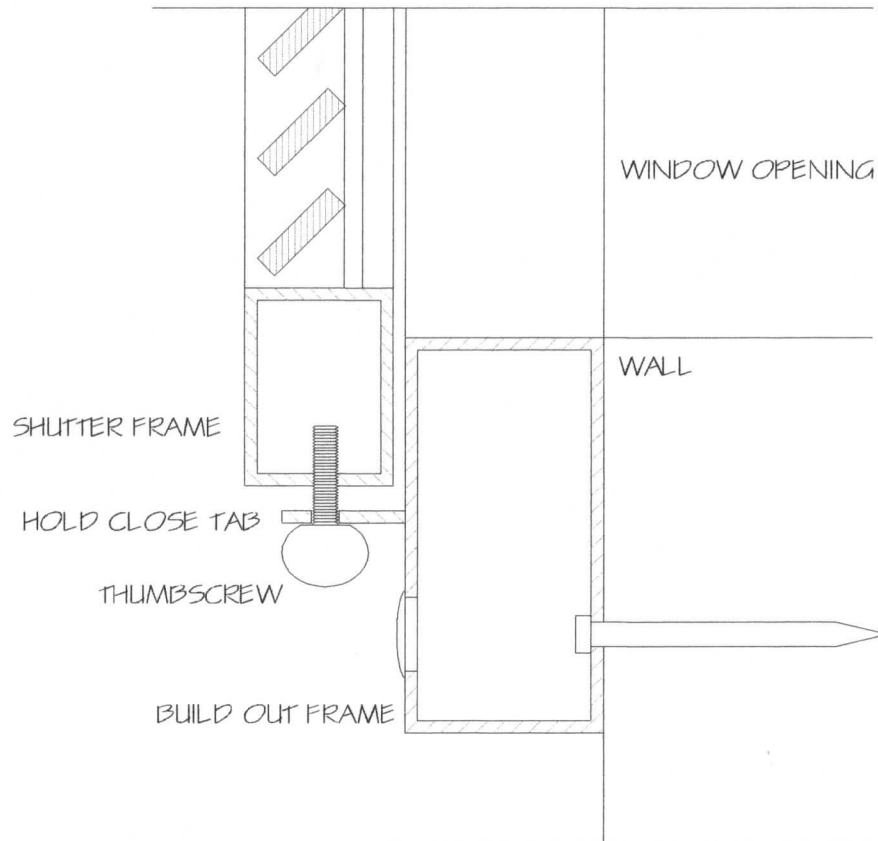
3 HURRICANE SHUTTER OUTSIDE CLOSURE BSI TAB on BUILD OUT FRAME with THUMBSCREW
