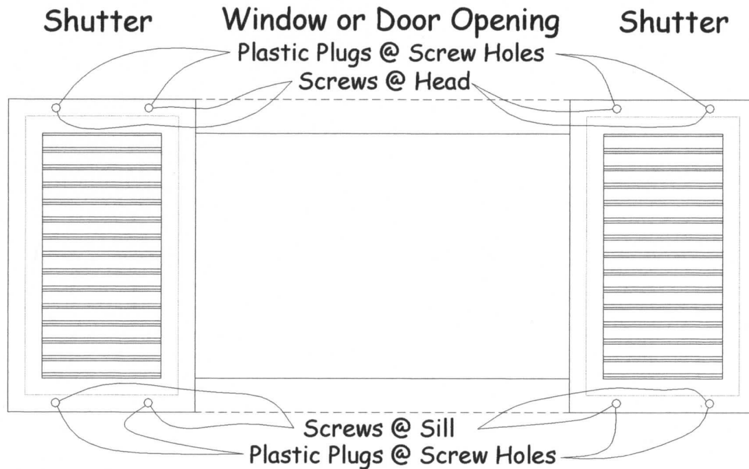
FIGURE 1 - ELEVATION
