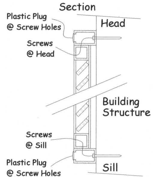
FIGURE 2 - SECTION
