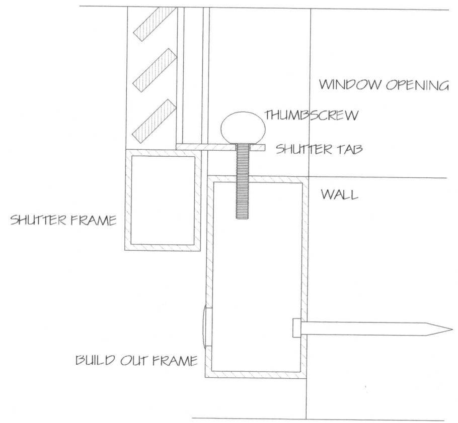
1 HURRICANE SHUTTER INSIDE BSI CLOSURE WITH THUMBSCREW
