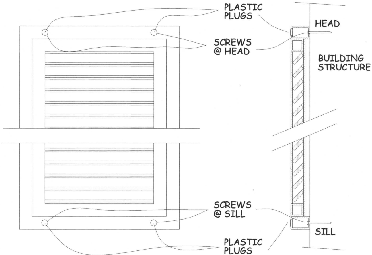
FIGURE 1 - ELEVATION
